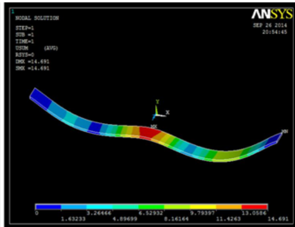
MAX DEFLECTION
