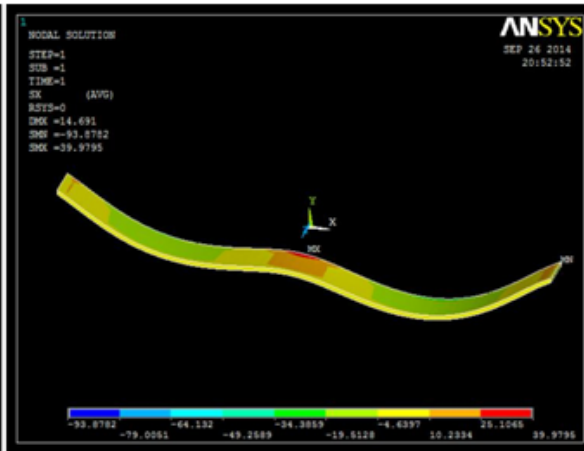
STRESS X-DIRECTION
