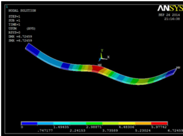
MAX DEFLECTION
